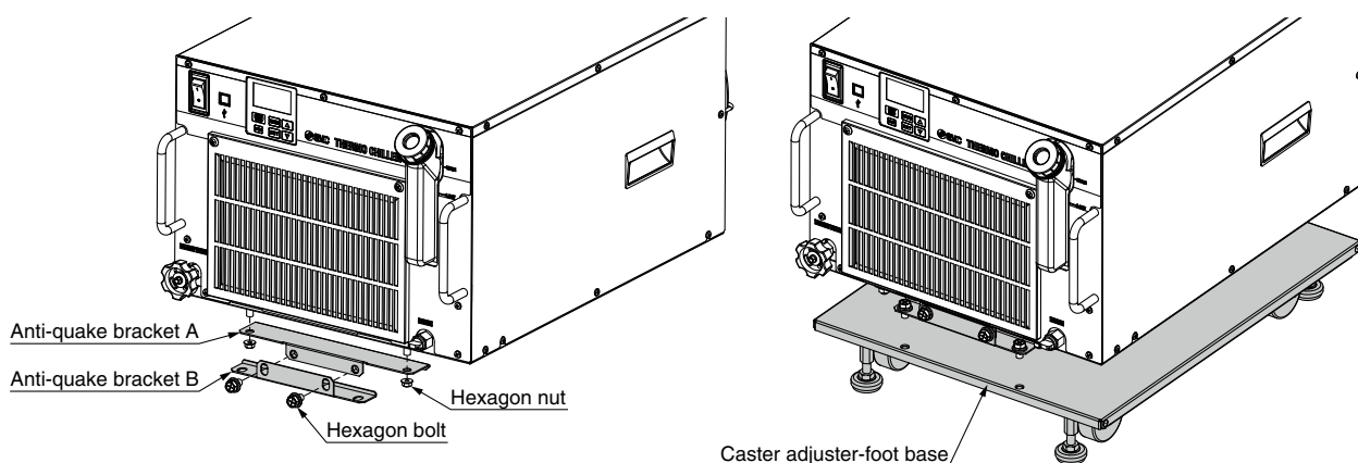
Mounting view
