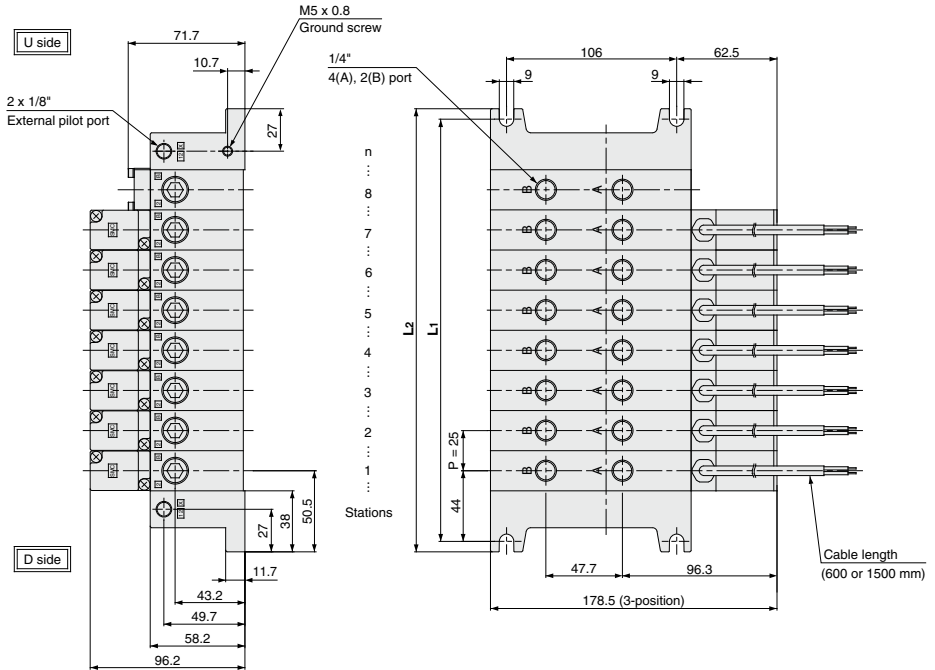
Bottom ported drawing
