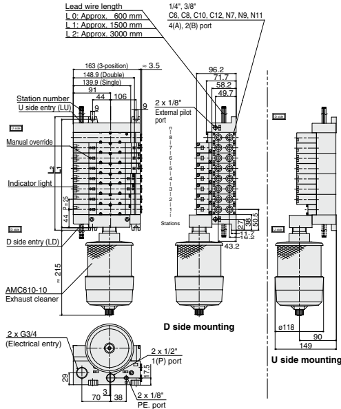
Plug-in type
