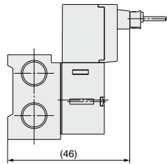
L plug connector (L)
