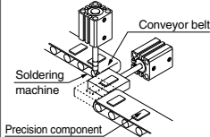
Transferring precision components
