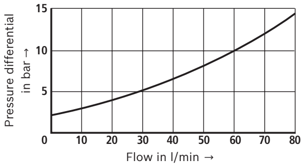
\Delta p - q_v characteristic curves
