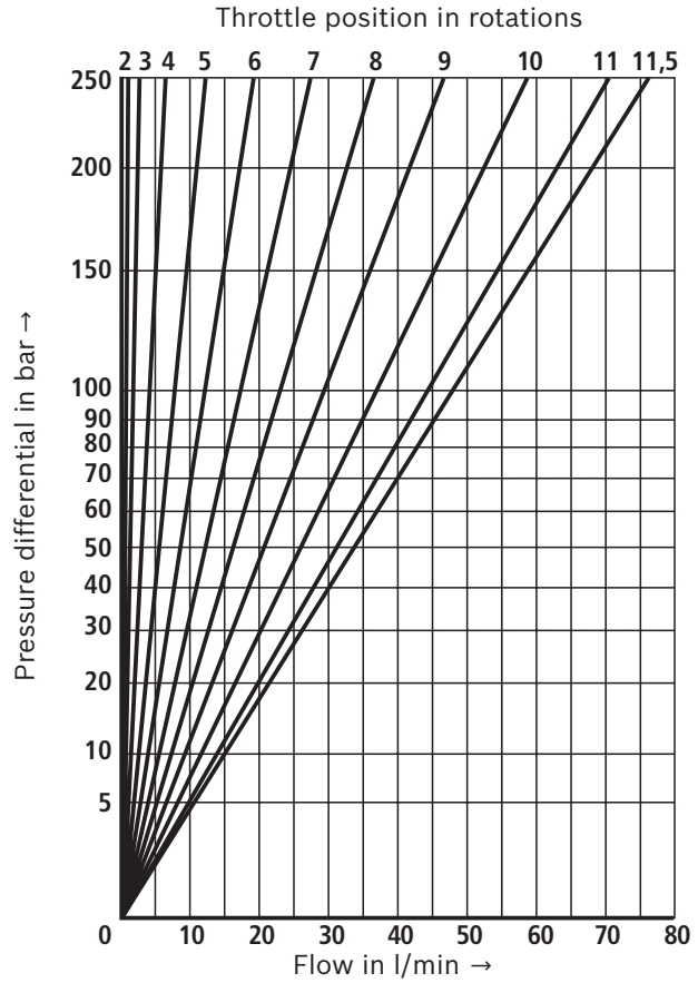
\Delta p - q_v characteristic curves (version "1Q")
